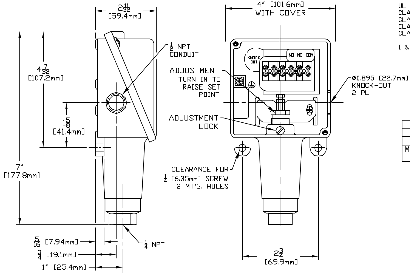
COVER REMOVED IN FRONT VIEW
